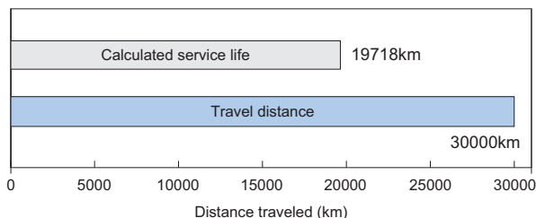
SHS65LVSS High-speed Durability Test Data
