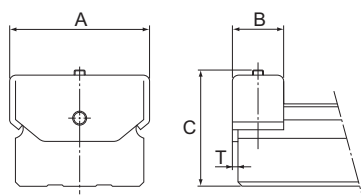
Fig.1 End Piece EP for Models NR/NRS
