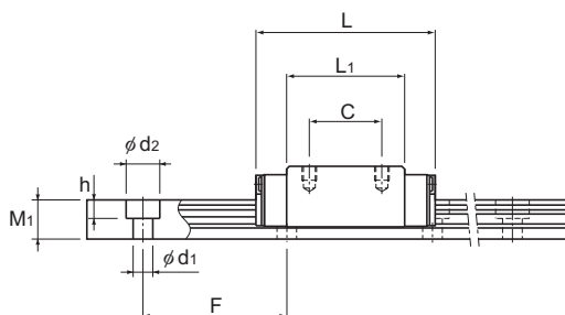
Models HSR8RM and 10RM
