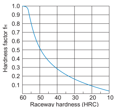
Fig.8 Hardness Factor ( f_H )
