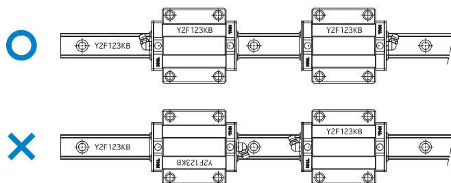
Fig.23 Serial Number Marking and Combined Use of an LM Rail and LM Blocks (E.g. Model HSR-A)
