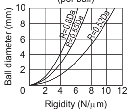
Comparison of rigidity by curvature (per ball)
