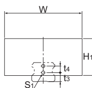
Models SHS15 to 30
