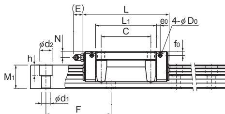
Models HSR45 to 85/LA
