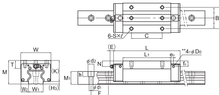
Models SRG25 to 30R/LR/LV
